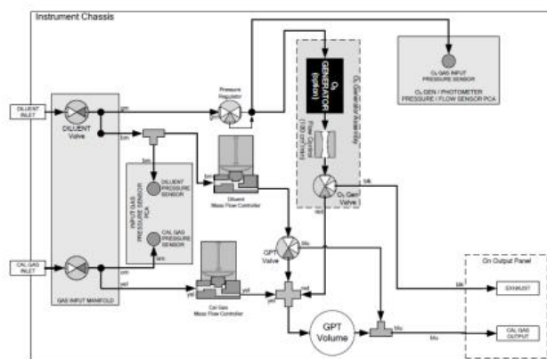
Figure 3-19: T750 Pneumatics with Optional O 3 Generator and GPT Chamber
