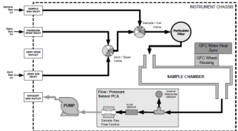
Figure 3-22: Internal Pneumatic Flow OPT 50A – Zero/Span Valves
